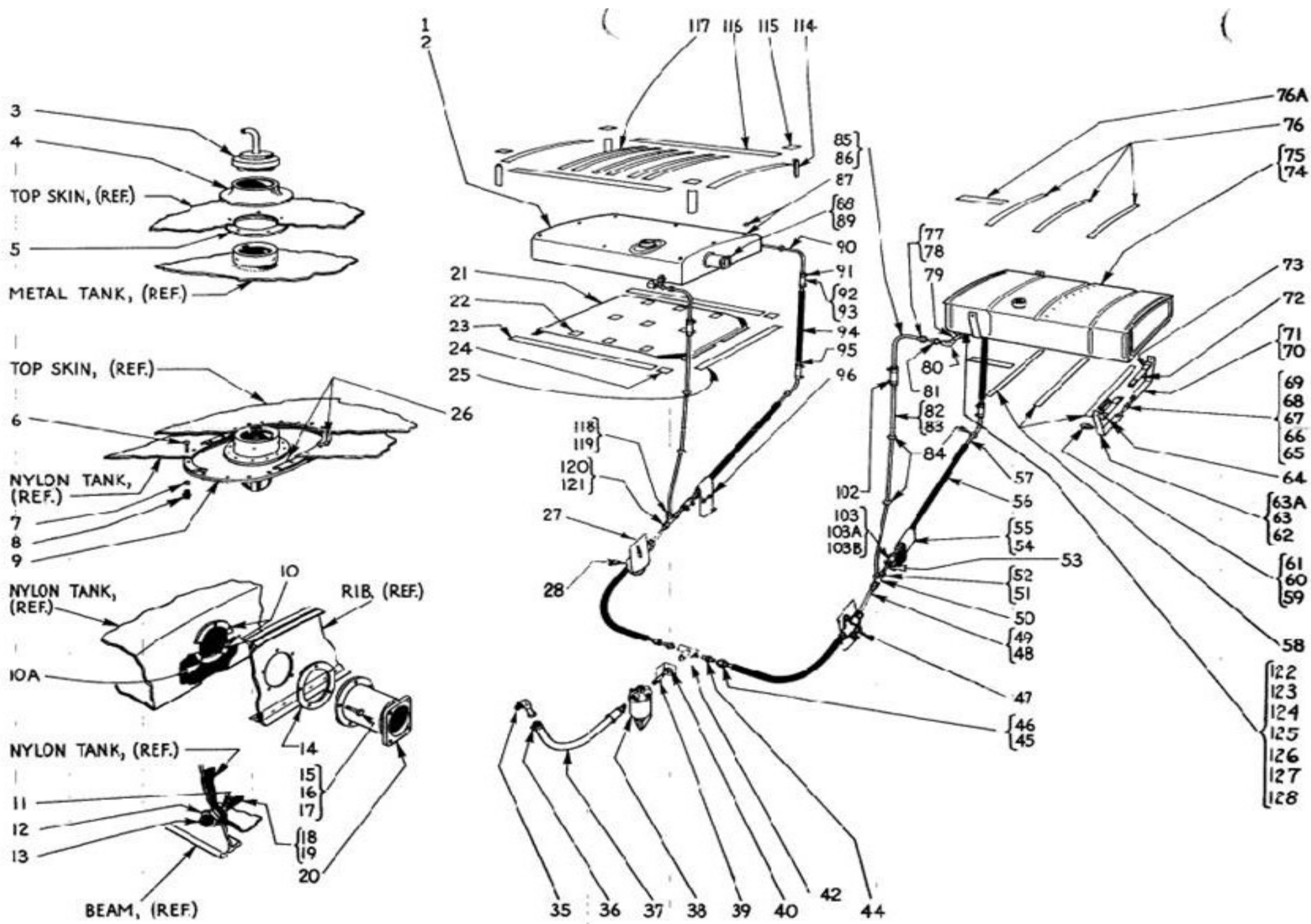
FIGURE No. 24 FUEL SYSTEM—WING TANKS
